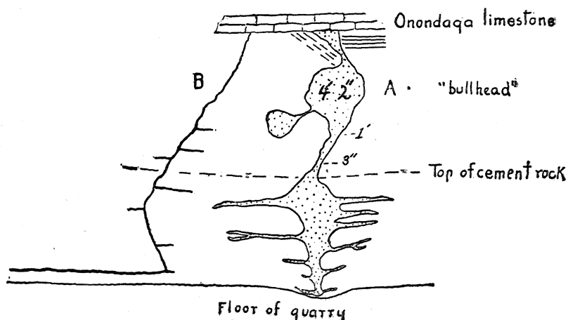
Diagram showing the largest of the sand dikes (A) in the quarries of the Buffalo cement co., at Buffalo N. Y. The floor of the quarry is the lowest layer used for burning cement and while the dike seems to enter this stratum it does not penetrate it. The figure shows the irregular character of the fissure walls, and the lateral apophyses in the lower part which are essentially parallel to the bedding. At the top is a slight displacement of the "bull-head" or Manlius waterlime on one side of the dike. B shows a second dike, the filling of a very narrow fissure. Others are evident elsewhere in this quarry. The Onondaga limestone lies horizontally over them all and is not penetrated by them.
