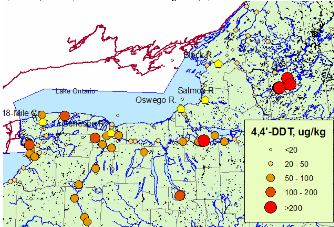
Figure 6. 4,4'-DDT in Great Lakes Basin surficial sediments.
